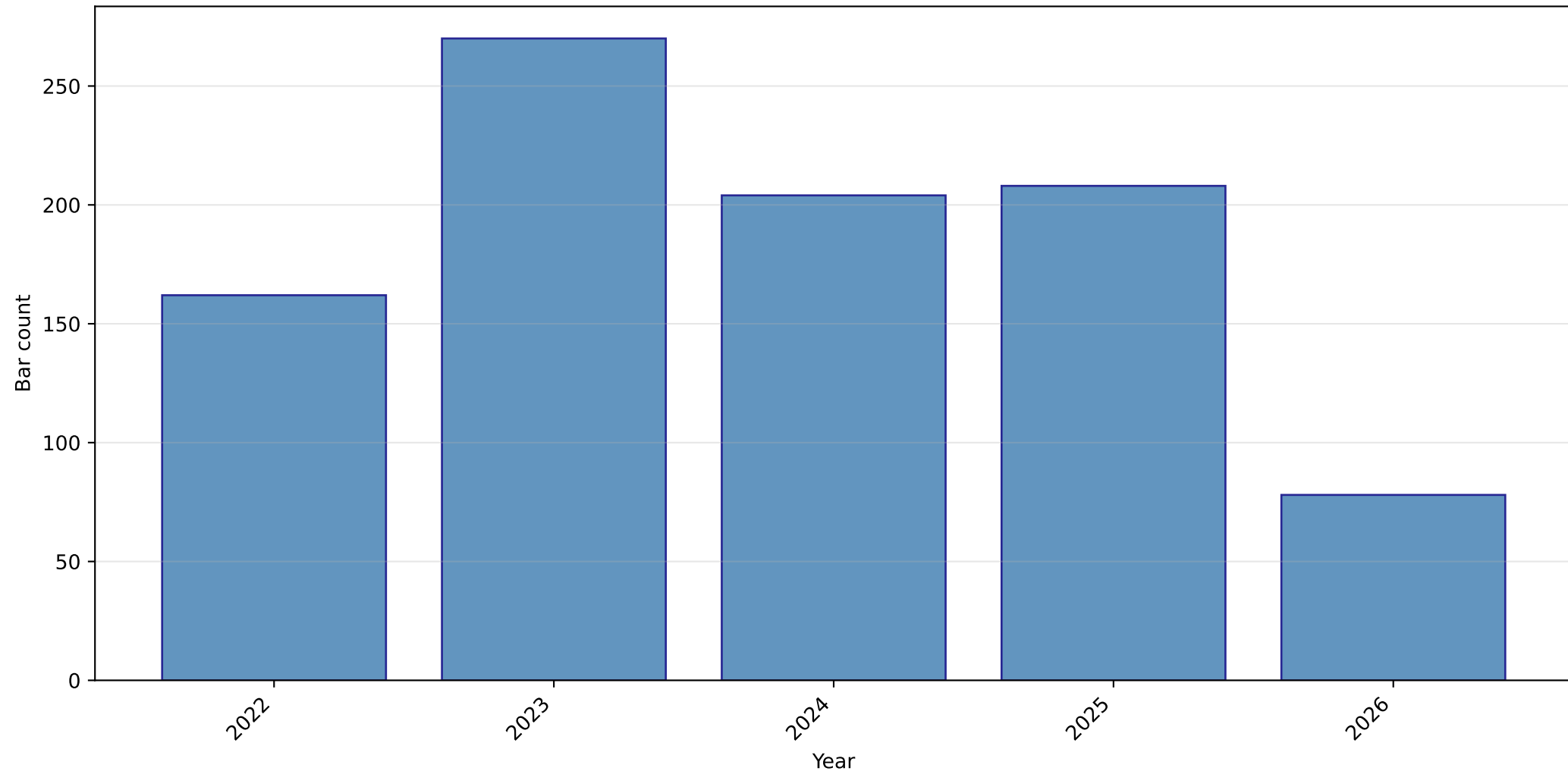
Regime 10 — bar counts by year (UTC) EURUSD · 60-minute bars (H1) · n=25,000 bars
