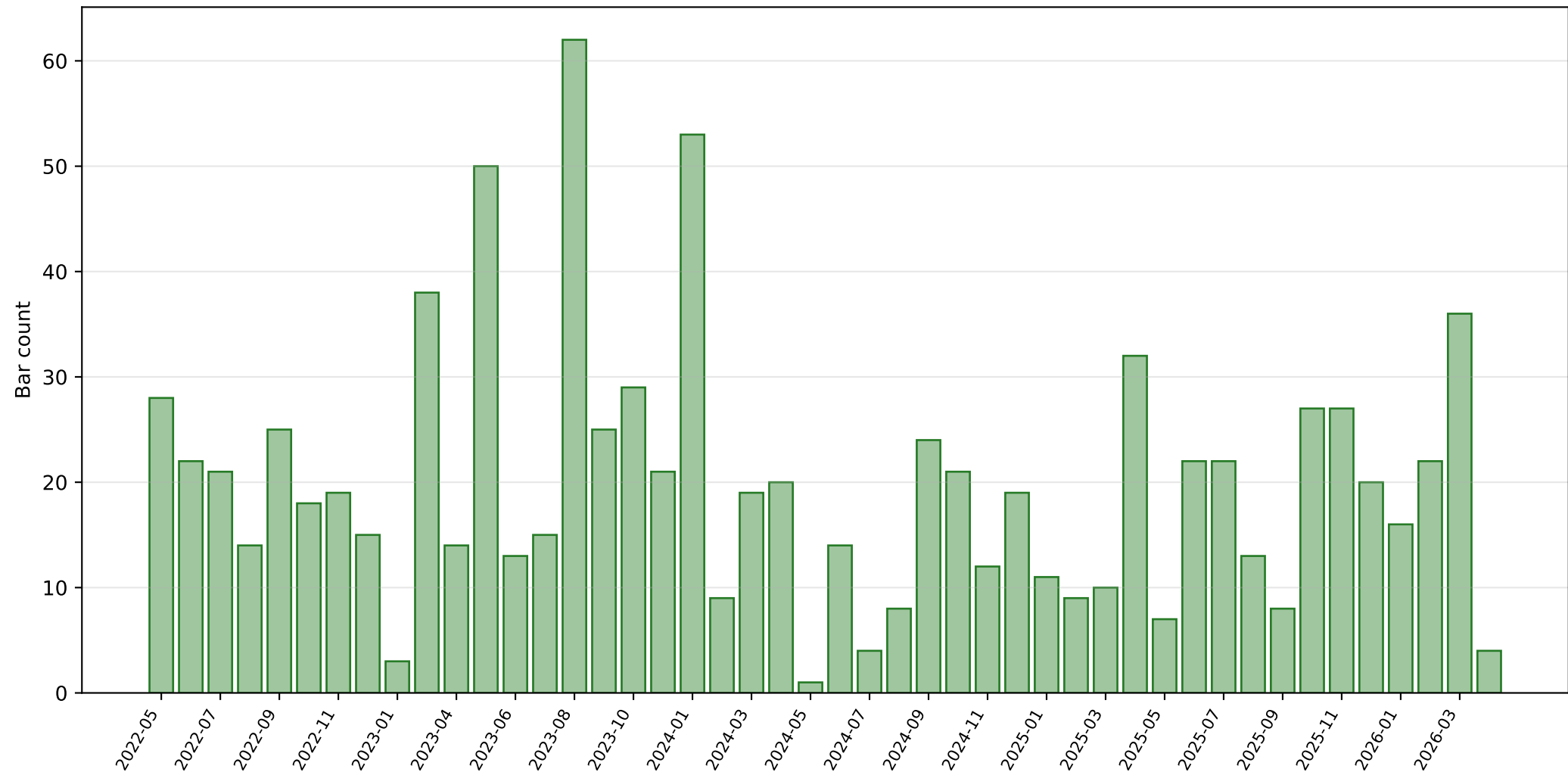
Regime 10 — bar counts by month (UTC, last 46 months) EURUSD · 60-minute bars (H1) · n=25,000 bars
