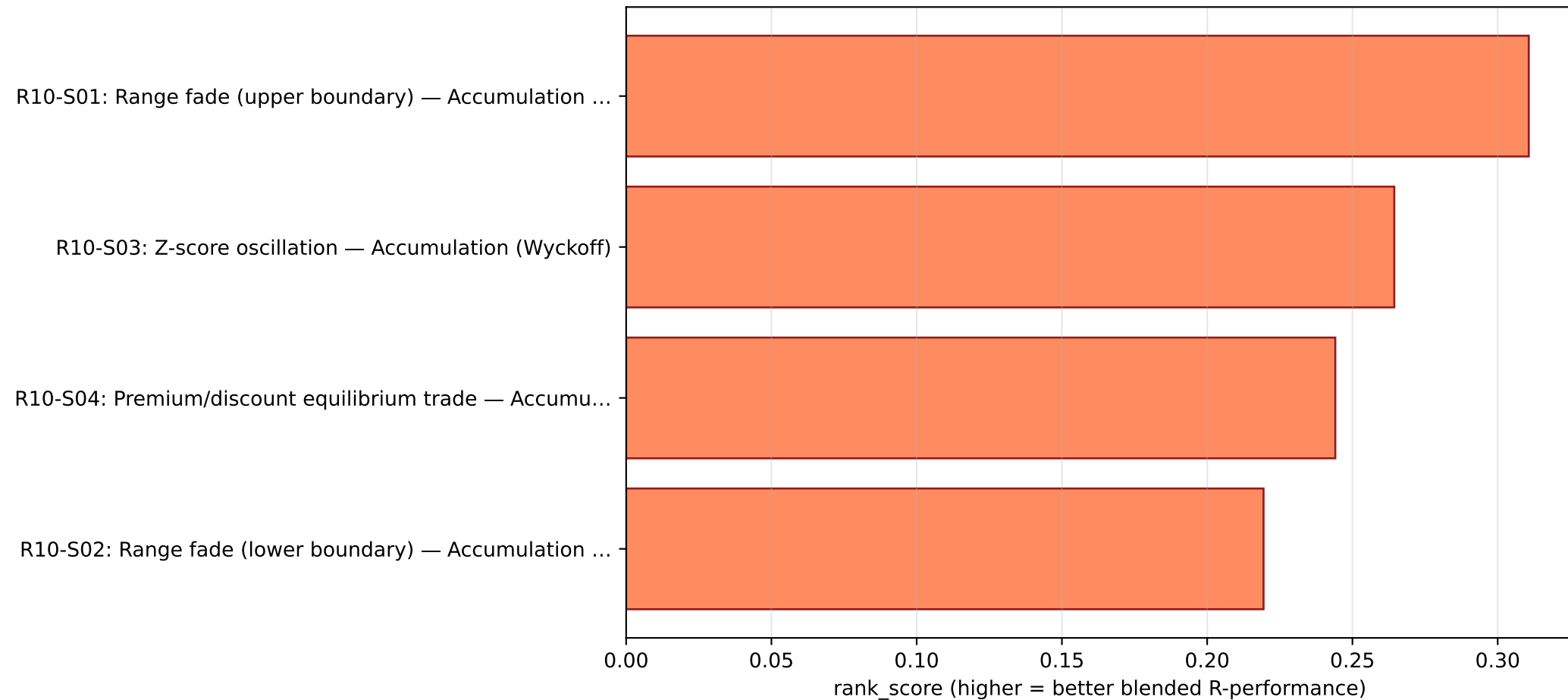
Top strategies by rank_score — regime 10 EURUSD · 60-minute bars (H1) · n=25,000 bars
